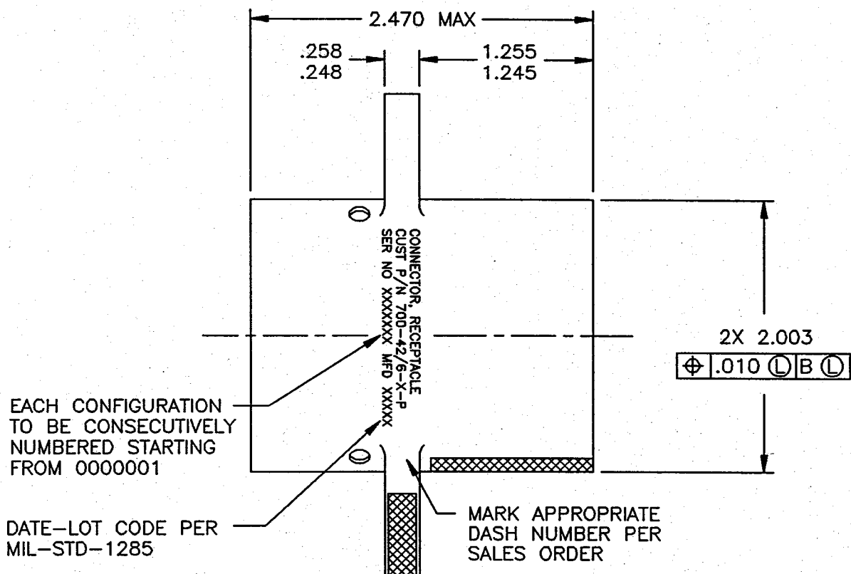
VIEW B-B
