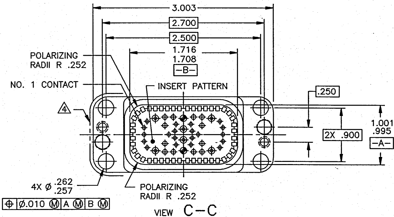
FIGURE 2A - CONNECTOR CONFIGURATION, RECEPTACLE, ELECTRICAL, RECTANGULAR (CONTD) (PAGE 2 OF 4)
